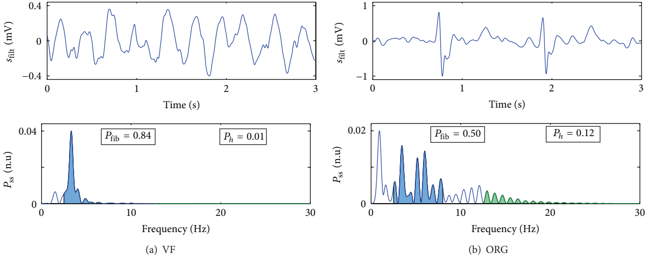
FIGURE 5: Example of the frequency domain analysis for VF (a) and an ORG (b) window. VF concentrates most of its power around the fibrillation band (blue). ORG rhythms have a spectrum with many harmonics of the heart rate and thus larger P_h (in green).
